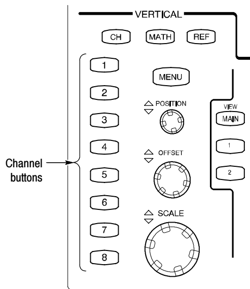
Figure 1- 15: Channel button location
