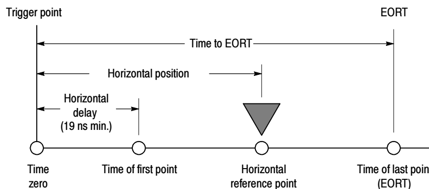
Figure 3-15: Trigger to End Of Record Time (EORT)
